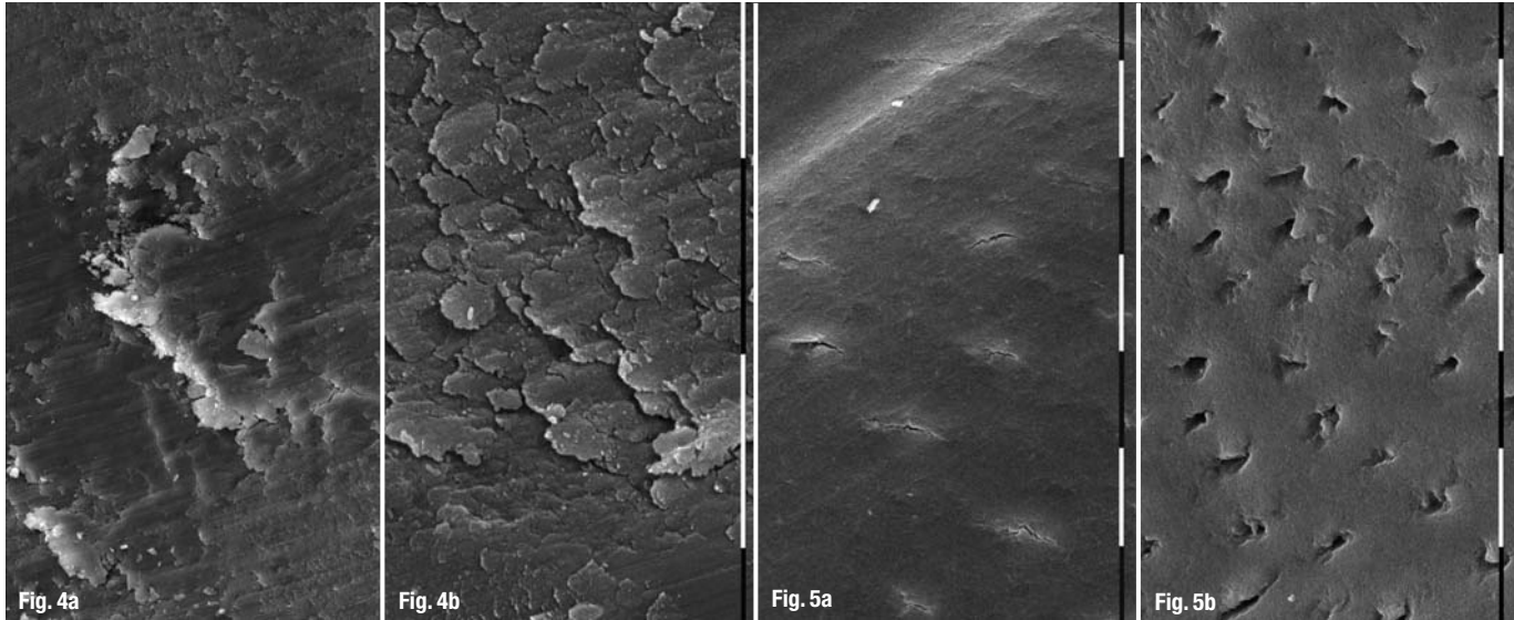
Figs. 4a & b SEM photomicrographs of tooth surfaces prepared with steel burs (x 500; 2,000 magnification). The surface is covered with a layer of debris and dental tubule orifices are not visible.
